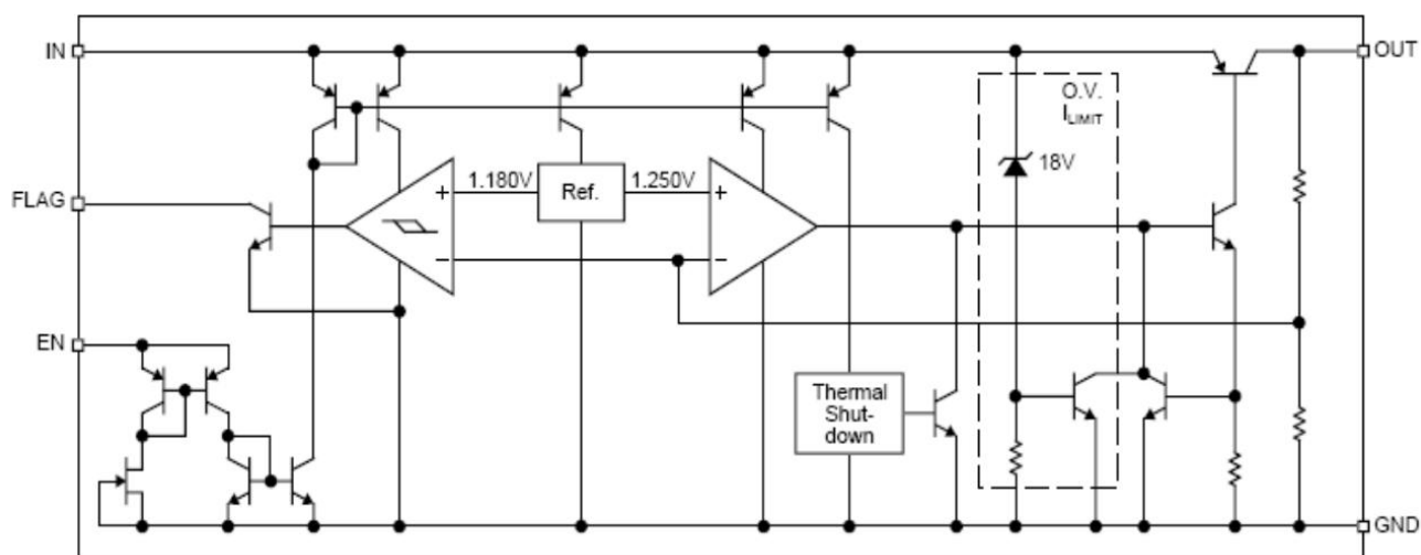
MIC39301 Fixed with flag and enable
