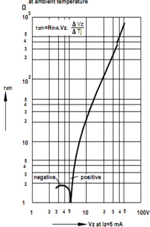
Thermal differential resistance versus Zener voltage
