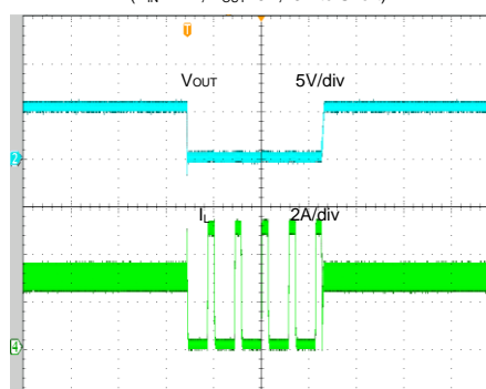
Short Circuit Protection ( V_{IN}=12V , V_{OUT}=5V , 3A to Short)
