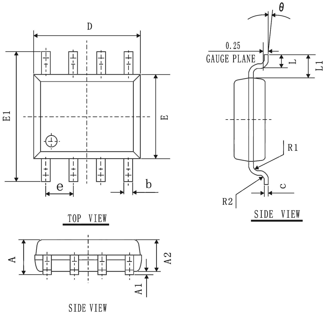
COMMON DIMENSIONS (UNITS OF MEASURE=mm)
