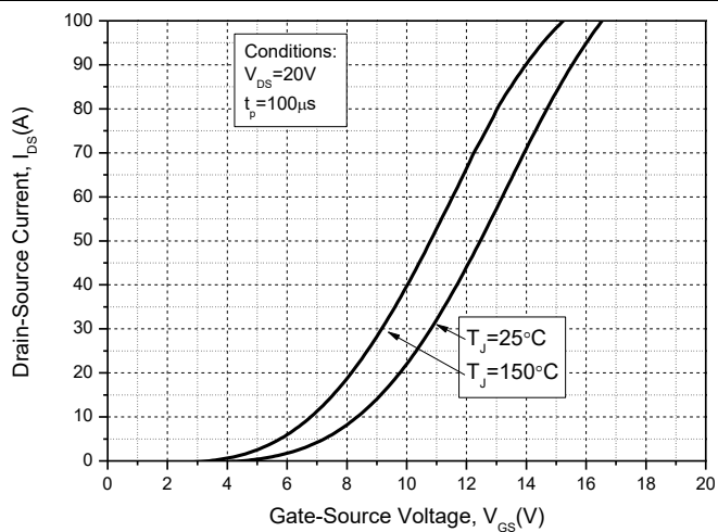
Figure 5. Transfer Characteristic
