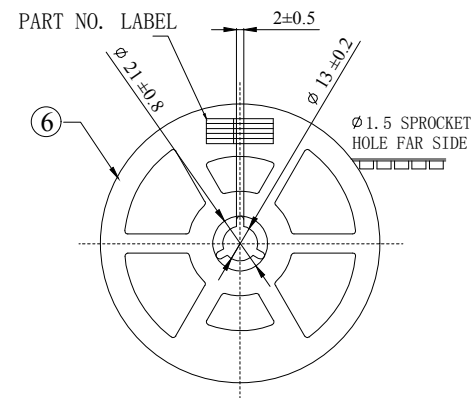
STYLE AND DIMENSION OF REEL PER REEL 15000 CONNECTORS
