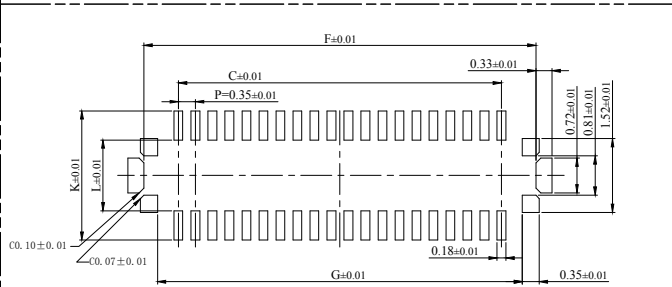
RECOMMENDED METAL DIMENSIONS (THICKNESS: 0.08 mm)
