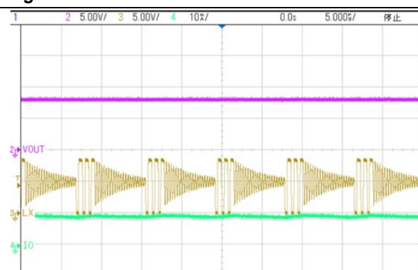
Figure 14.3.b V_{\text{IN}}=5\text{V} , I_{\text{OUT}}=10\text{mA} , 3pcs LED Series
