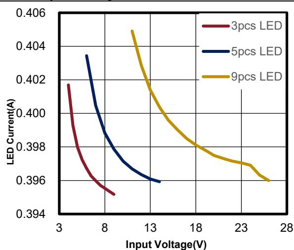
Figure 12.2.b I_{OUT}=400mA
