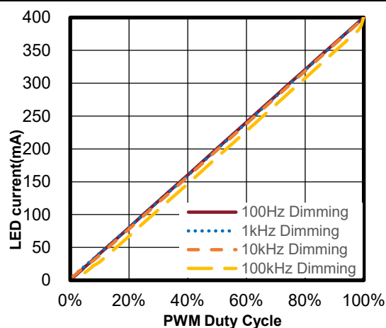
Figure 13.2.e LGS63032, V_{IN}=5V , 3pcs LED Series
