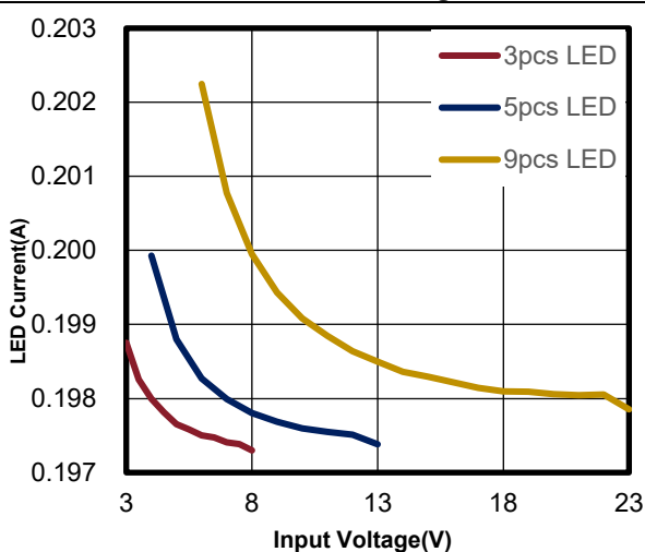
Figure 12.2.a I_{OUT}=200mA
