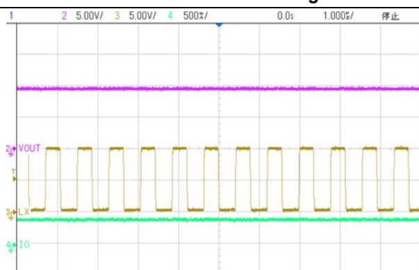
Figure 14.3.a V_{\text{IN}}=5\text{V} , I_{\text{OUT}}=400\text{mA} , 3pcs LED Series
