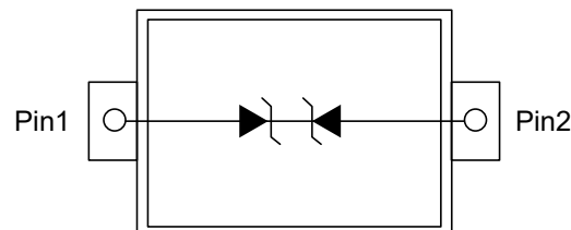
SOD-323
