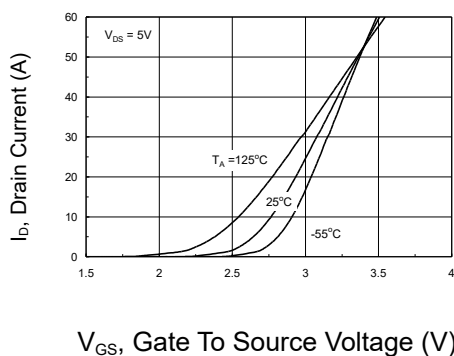
Figure 5: Transfer Characteristics
