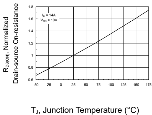
Figure 3: On-Resistance Variation with Temperature
