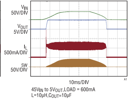
Power Up and Power Down EN = VIN
