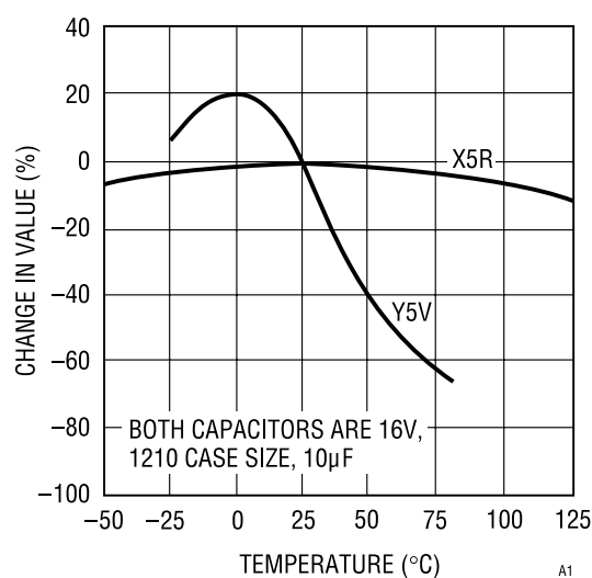
Figure17.b. Ceramic Capacitor DC Bias Characteristics
