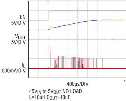
Start-Up Waveforms NO LOAD
