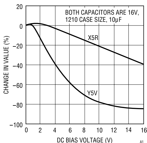
Figure17.a Ceramic Capacitor DC Bias Characteristics
