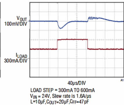
Load Transient, V_{\text{OUT}} = 5\text{V}
