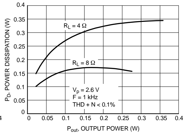
Figure 34. Power Dissipation versus Output Power
