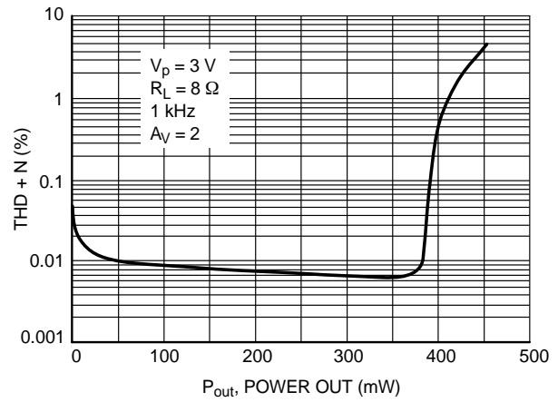
Figure 8. THD + N versus Power Out
