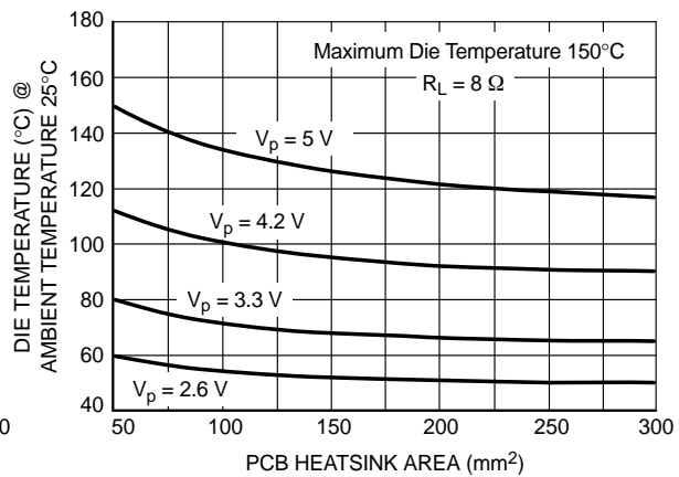
Figure 36. Maximum Die Temperature versus PCB Heatsink Area
