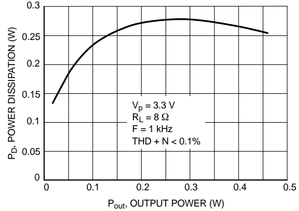
Figure 32. Power Dissipation versus Output Power
