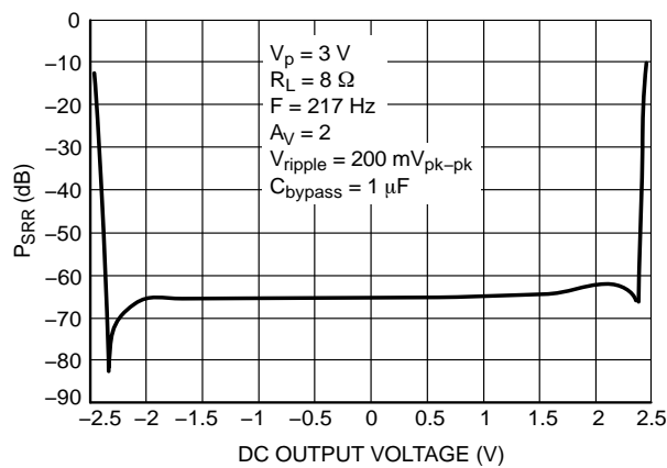
Figure 27. PSRR @ DC Output Voltage
