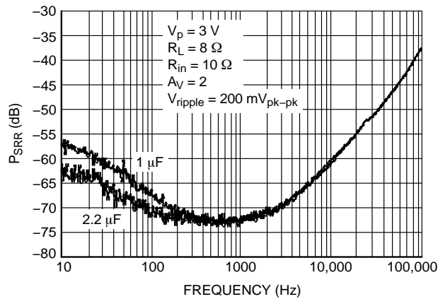
Figure 25. PSRR versus C_{bypass} @ V_p = 3\text{ V}
