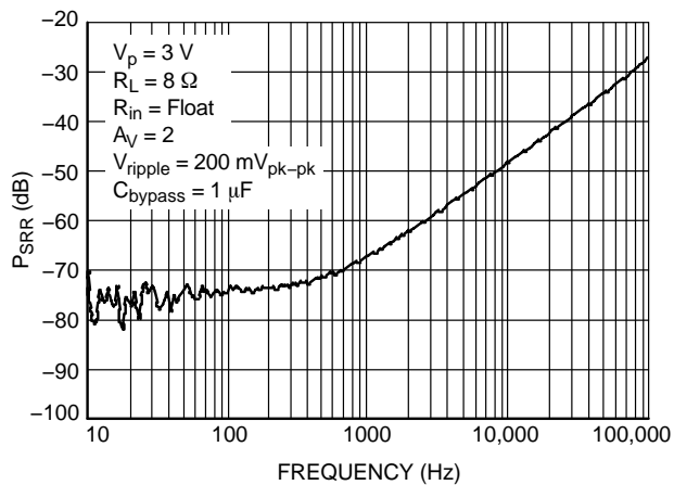
Figure 17. P_{\text{SRR}} @ V_p = 3\text{ V}
