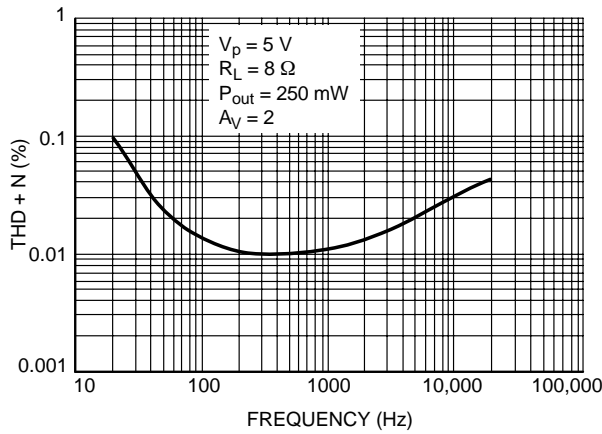
Figure 1. THD + N versus Frequency
