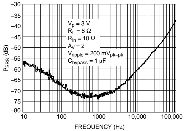
Figure 16. P_{\text{SRR}} @ V_p = 3\text{ V}
