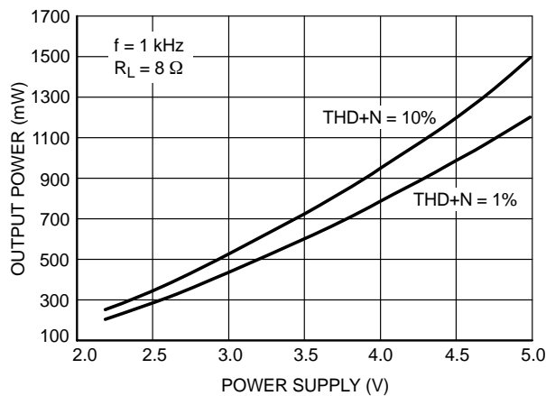
Figure 11. Output Power versus Power Supply
