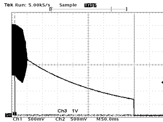
Figure 30. Turning Off Time - V_p = 5\text{ V}
