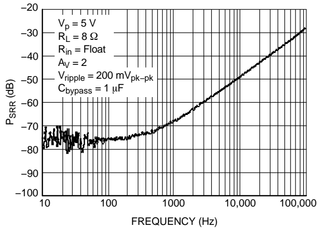
Figure 13. P_{\text{SRR}} @ V_p = 5\text{ V}
