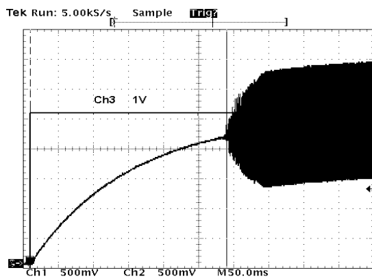
Figure 29. Turning On Time - V_p = 5\text{ V}
