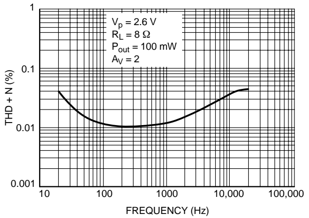
Figure 4. THD + N versus Frequency
