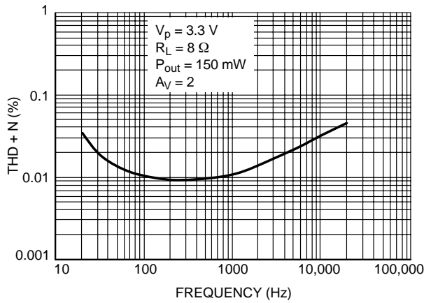
Figure 2. THD + N versus Frequency
