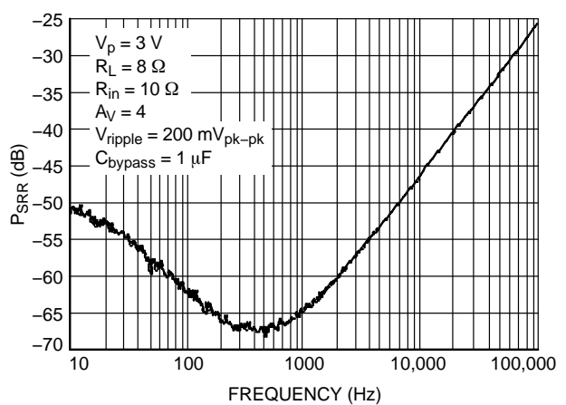
Figure 18. P_{\text{SRR}} @ V_p = 3\text{ V}
