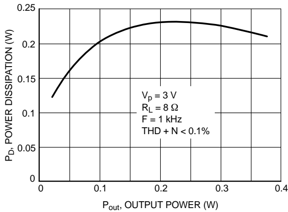
Figure 33. Power Dissipation versus Output Power
