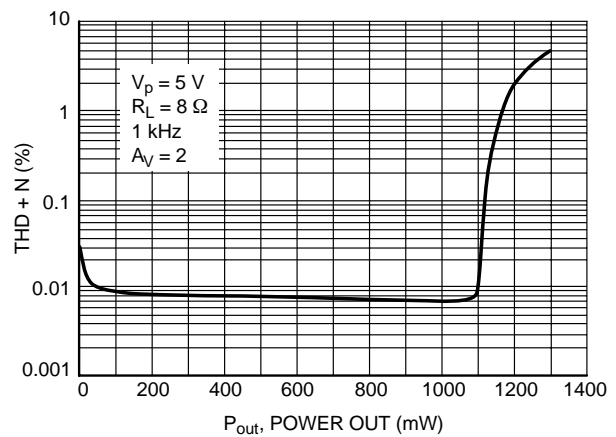
Figure 6. THD + N versus Power Out
