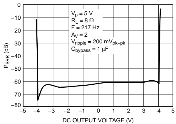
Figure 26. PSRR @ DC Output Voltage
