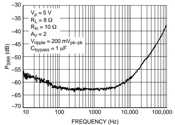
Figure 12. PSRR @ V_p = 5 \text{ V}
