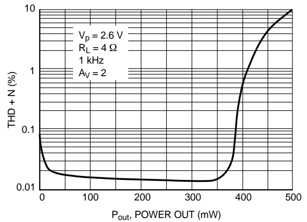
Figure 10. THD + N versus Power Out
