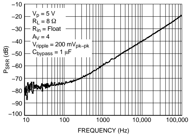
Figure 15. P_{\text{SRR}} @ V_p = 5\text{ V}
