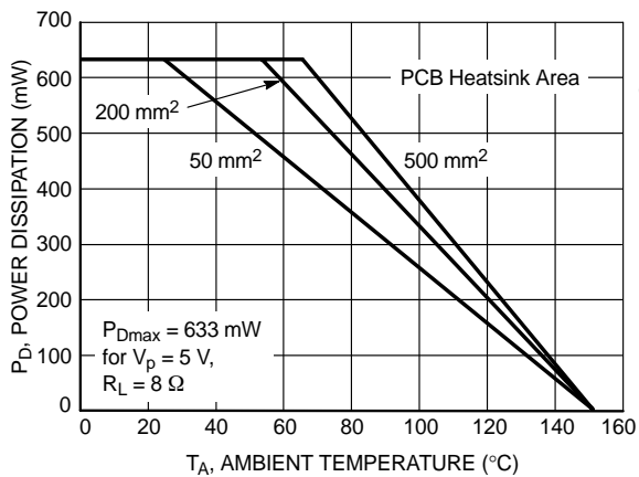
Figure 35. Power Derating – 9-Pin Flip-Chip CSP
