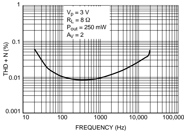
Figure 3. THD + N versus Frequency
