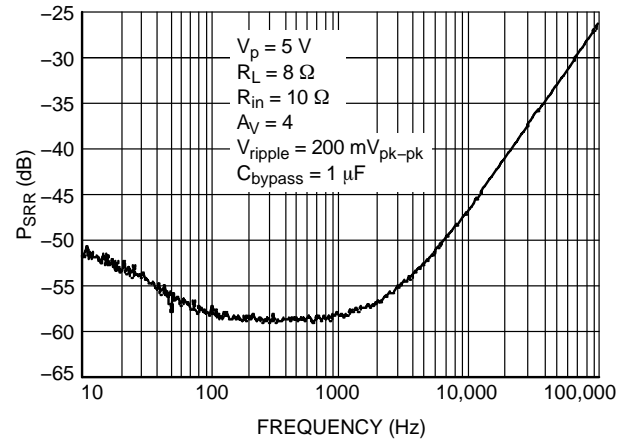
Figure 14. P_{\text{SRR}} @ V_p = 5\text{ V}
