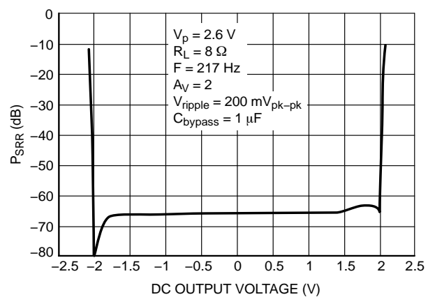
Figure 28. PSRR @ DC Output Voltage
