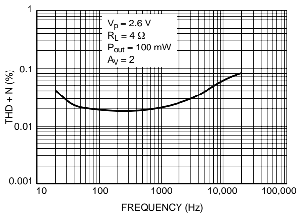
Figure 5. THD + N versus Frequency
