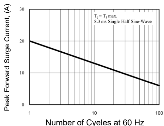
Figure 2: Maximum Non-Repetitive Surge Current
