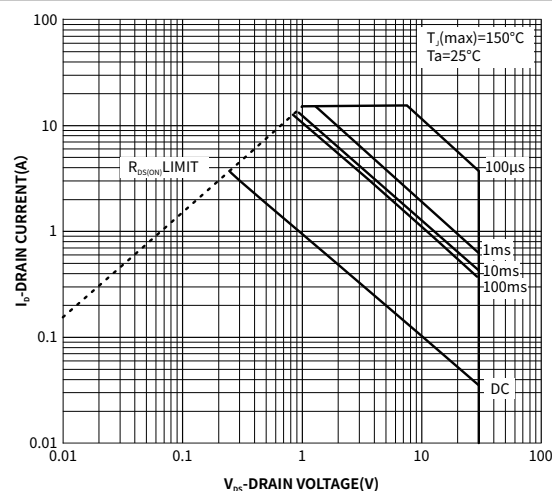
Fig.8 Safe Operation Area
