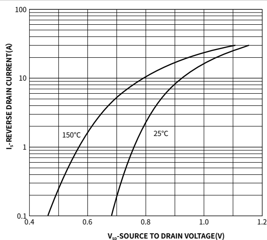
Fig.7 Diode Characteristics
