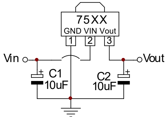
1. Basic circuit
