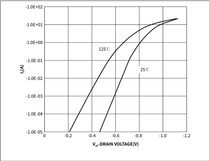
Fig.7 Diode Characteristics
