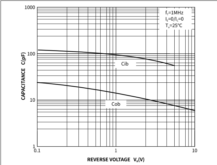
Fig.6 Cob/Cib- V_{CB} V_{BE}
