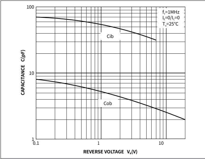
Fig.6 Cob/Cib- V_{sV_{eb}}
