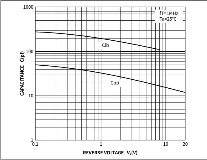
Fig.6 Cob/Cib- V_{cb}
