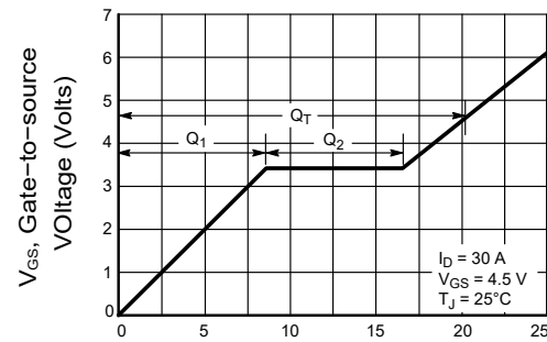
Q_G , Total Gate Charge (nC)
