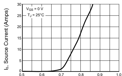
V_{SD} , Source-to-drain Voltage (VOLTS)
