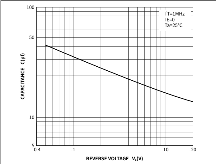
Fig.6 Cob/Cib- V_{CB}V_{EB}
