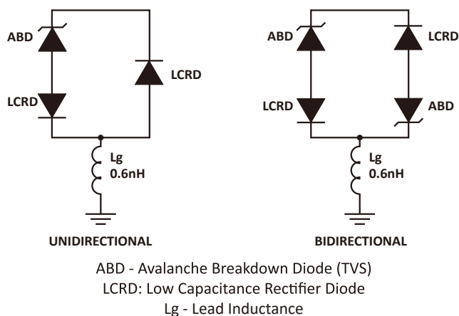
FIGURE 1 SPICE MODEL
