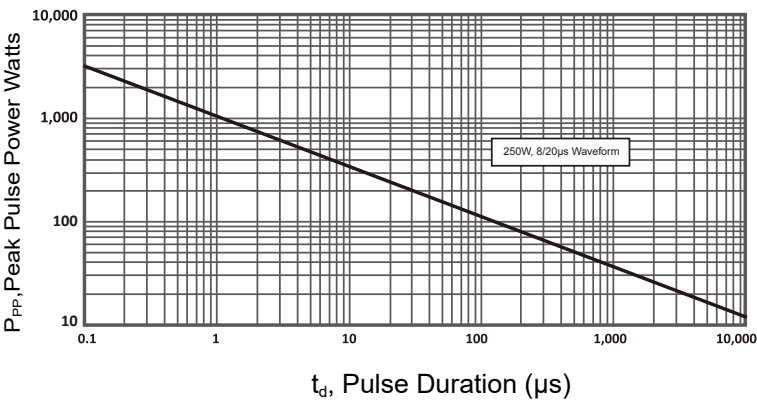
Figure 1: Peak Pulse Power Vs Pulse Time
