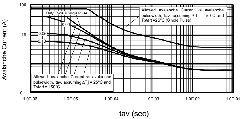
Figure 20: Typical Avalanche Current vs.Pulse width
