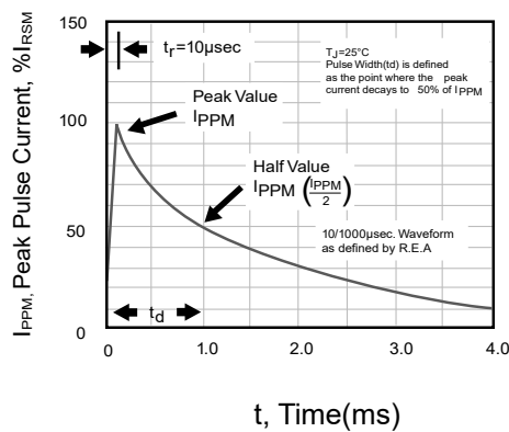
Figure 3: Pulse Waveform
