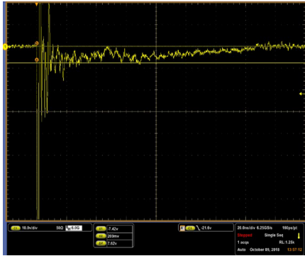
Figure 16: AQHV24 -8kV Contact ESD Clamping Voltage
