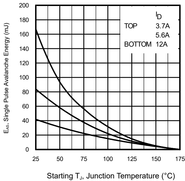
Figure 9: Maximum Avalanche Energy Vs. Drain Current
