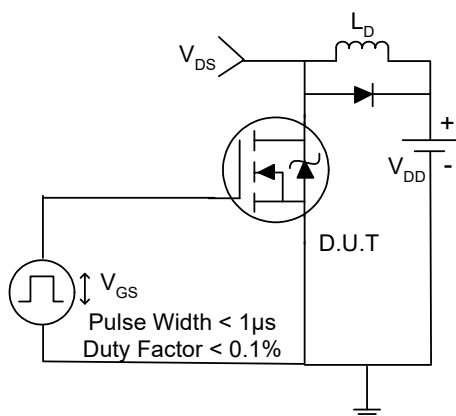
Figure 15: Gate Charge Test Circuit
