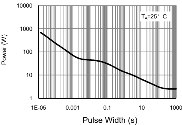
Figure 14: Single Pulse Power Rating Junction-to-Ambient (Note H)
