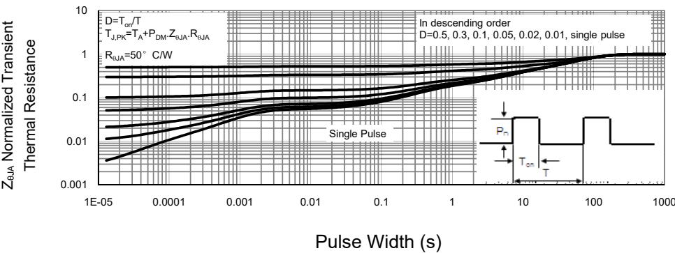
Figure 15: Normalized Maximum Transient Thermal Impedance (Note H)
