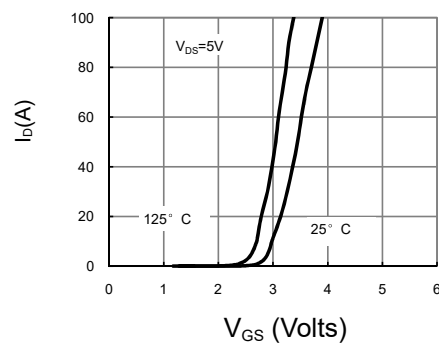
Figure 2: Transfer Characteristics (Note E)
