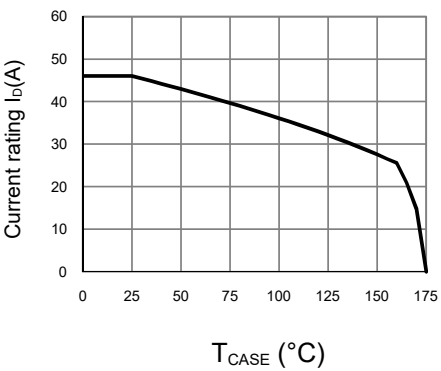
Figure 13: Current De-rating (Note F)
