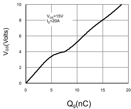
Figure 7: Gate-Charge Characteristics
