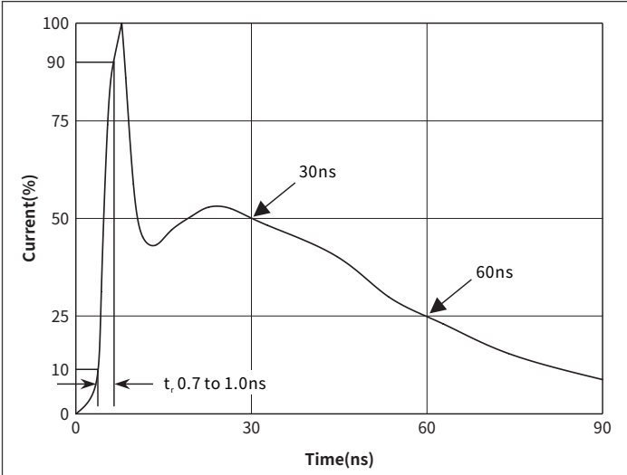
Fig.2 Pulse Waveform-ESD(IEC61000-4-2)
