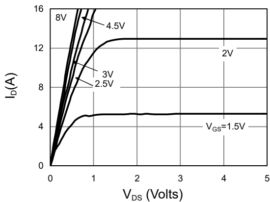
Fig 1: On-Region Characteristics
