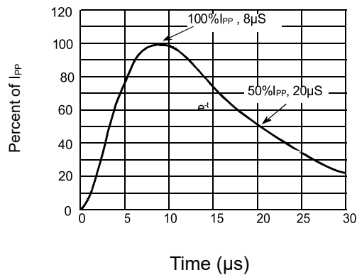
Figure 3: Pulse Wave form-8/20μs
