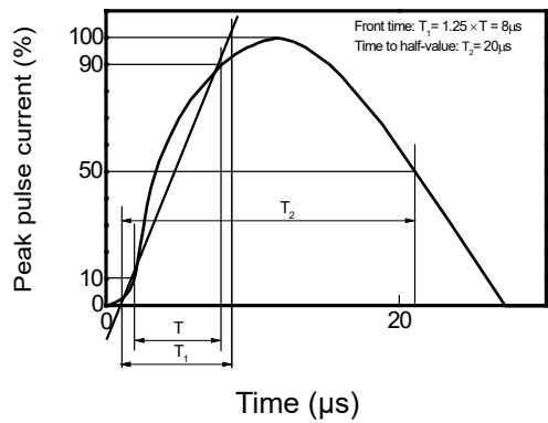
Figure 1: 8/20μs waveform per IEC61000-4-5
