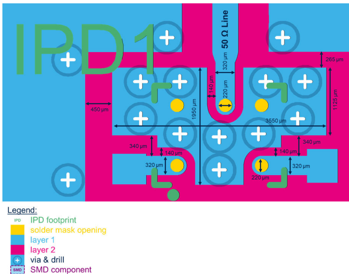
Figure 11. PCB land pattern recommendations
