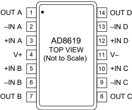
TSSOP-14/SOP-14
