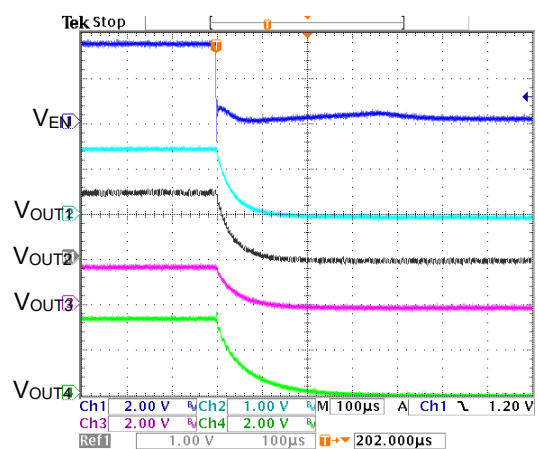
1A Loading EN Turn Off Waveform
