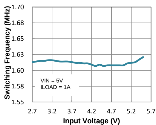
Freq. vs. Vin
