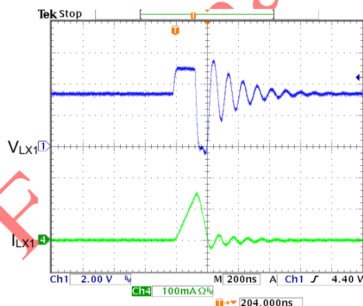
No Load LX Waveform
