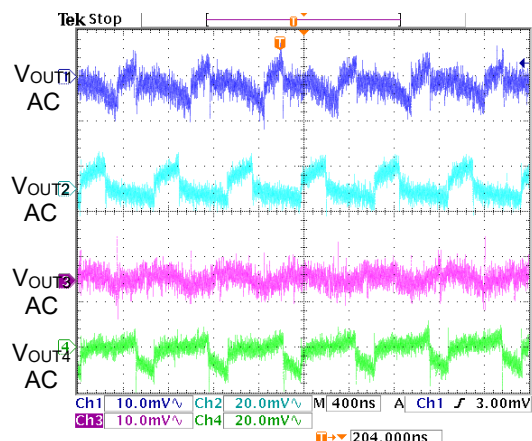
1A Loading Steady State Waveform
