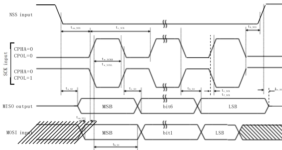
图 5: SPI 时序图-Slave Mode (CPHA = 0, CPOL=1)
