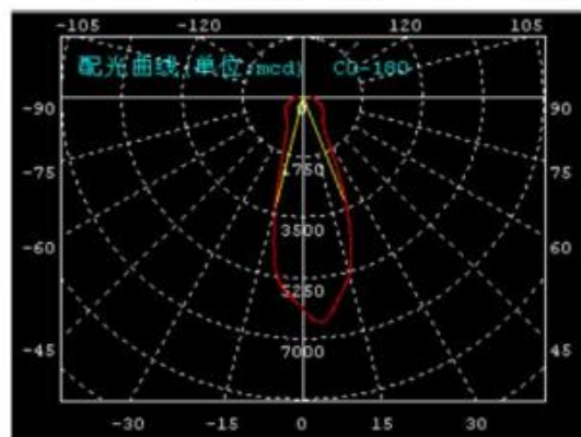
Light intensity distribution curve
