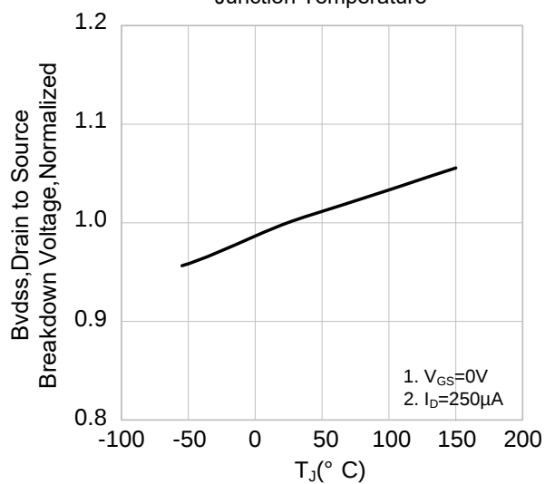
Typical Breakdown Voltage vs Junction Temperature
