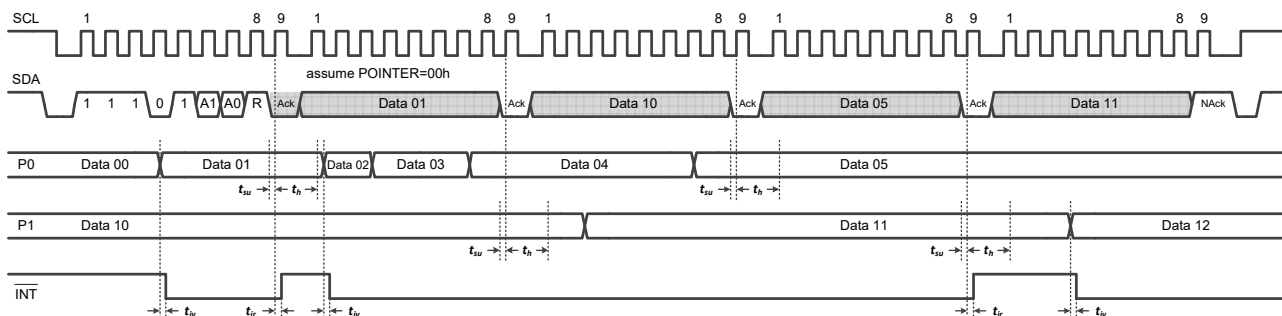
Figure 8. Read Input Port Registers, Scenario 1
