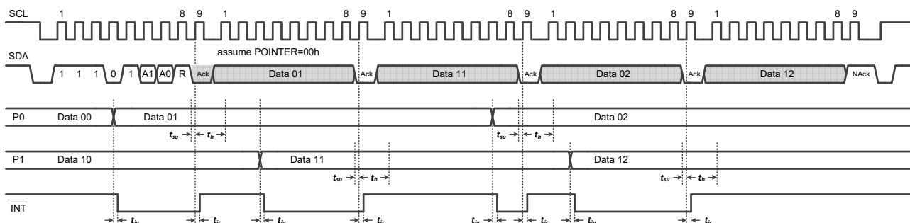
Figure 9. Read Input Port Registers, Scenario 2
