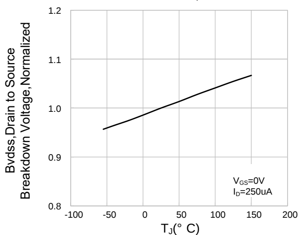
Typical Breakdown Voltage vs Junction Temperature
