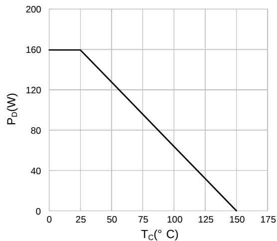
P_D vs. Temperature
