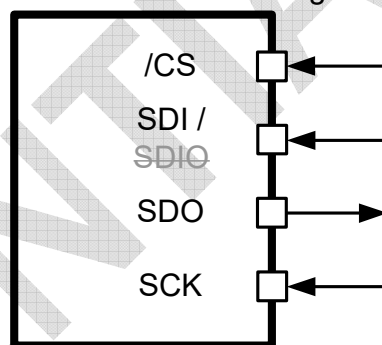
4- Wire SPI Connection Diagram
