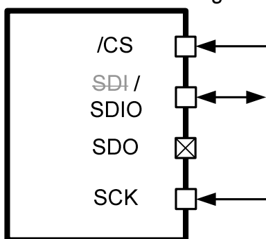
3- Wire SPI Connection Diagram
