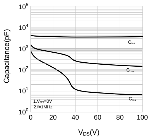
Capacitance Characteristics
