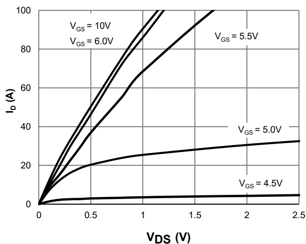
Saturation Characteristics
