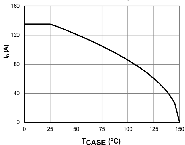
Current De-rating
