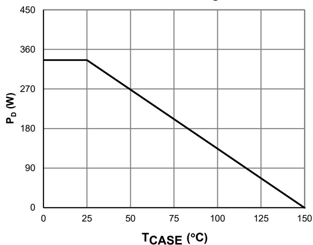
Power De-rating
