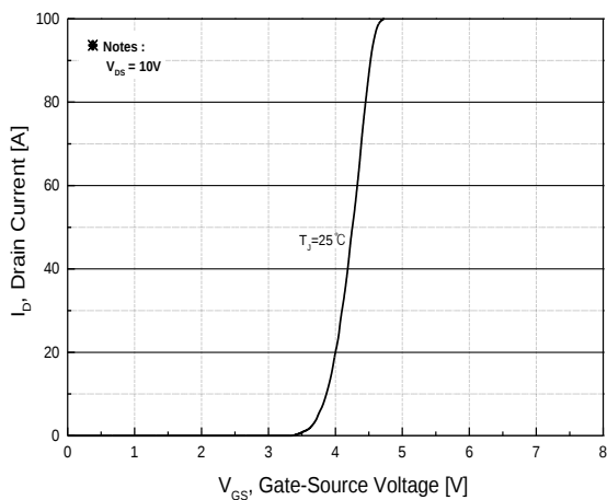
Fig.5 Transfer Characteristics
