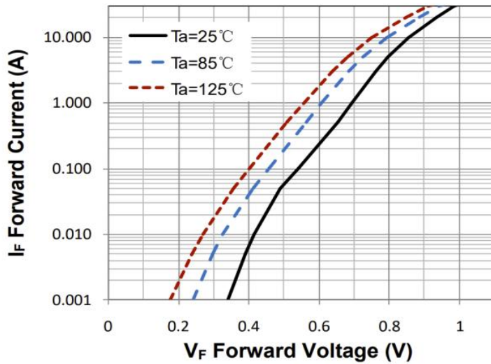
Figure 1. Forward Characteristic(typ.)
