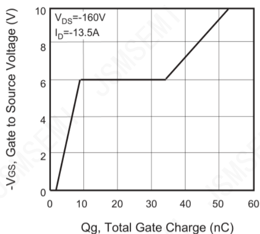
Figure 7. Gate Charge
