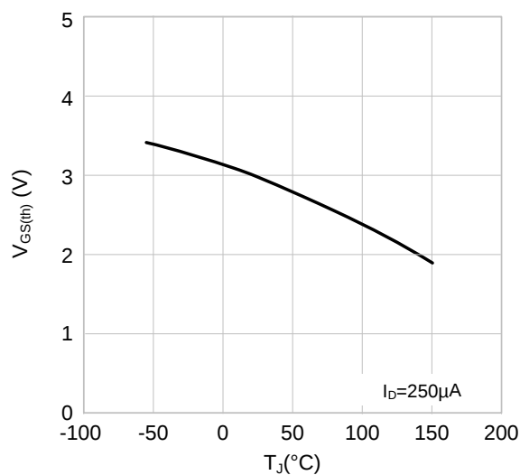
V_{GS(th)} vs T_J
