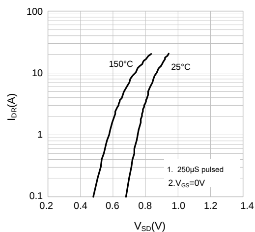
Body-diode Forward Characteristics
