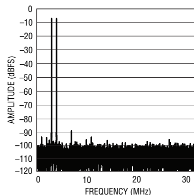
LTC2258-12 2-Tone FFT, f_{IN} = 68\text{MHz} and 69\text{MHz}
