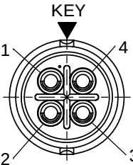
WIRING END W6382-4PG-P-3XX
