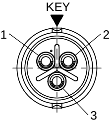
WIRING END W6382-3PG-P-3XX
