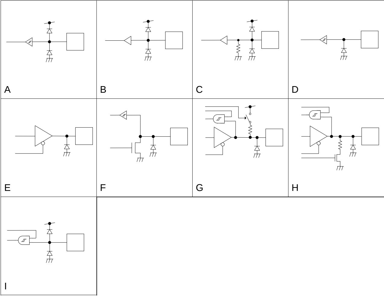
Fig.9 Equivalent I/O circuit diagram
