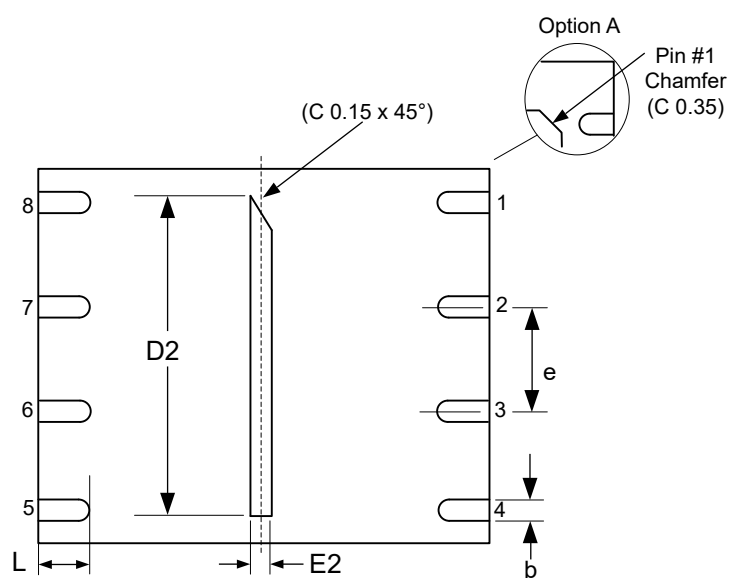
BOTTOM VIEW
